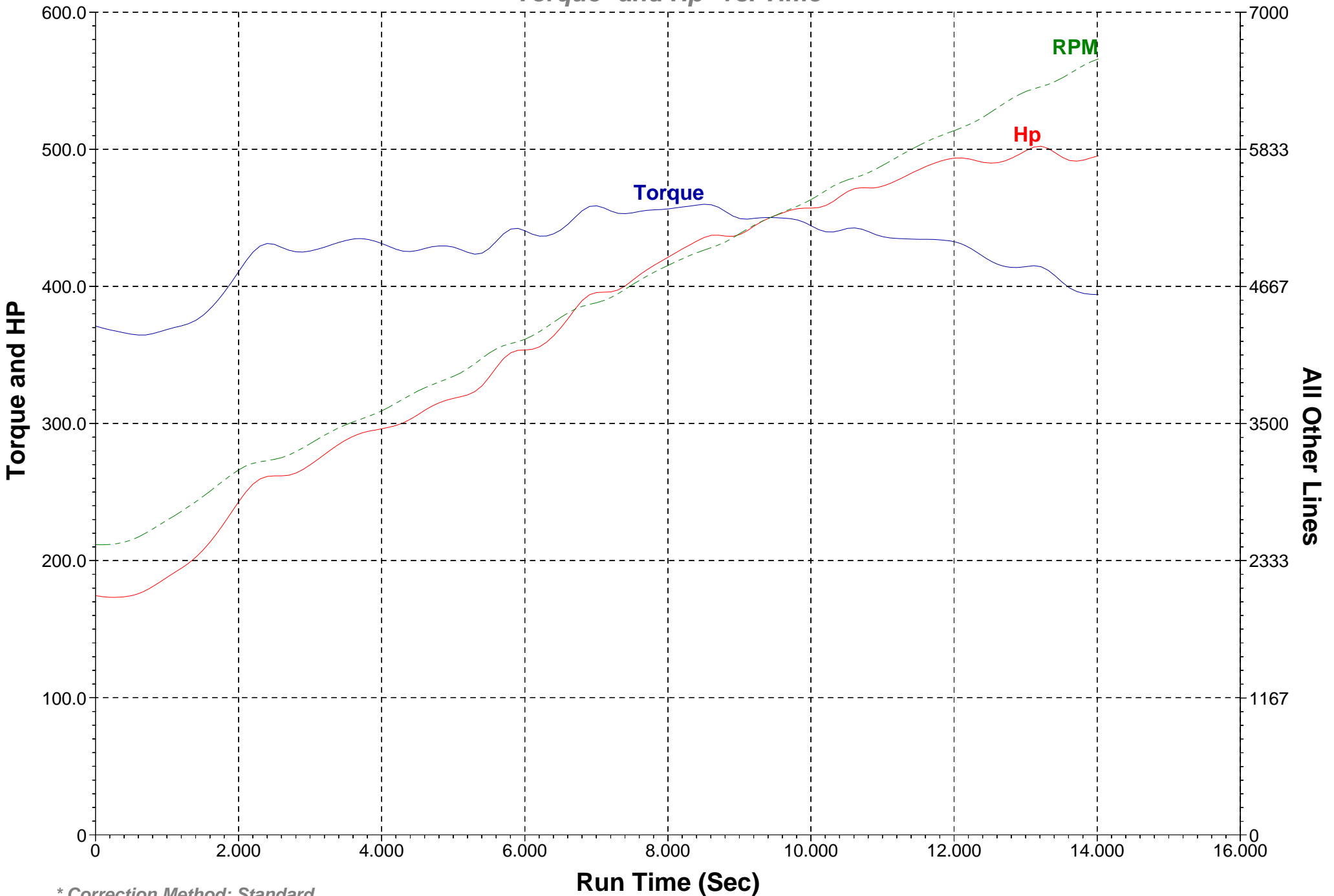
Torque* and Hp* vs. Time
